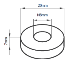
TERMINAL DIMENSION
